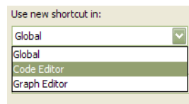
Figure 6 Shortcut context
